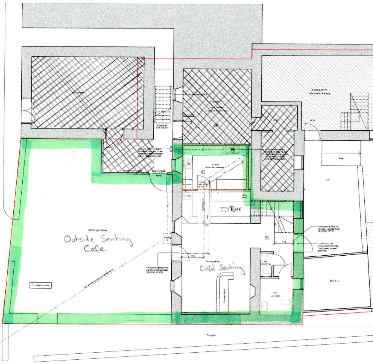
Proposed Ground Floor Detail & Services Plan 1:50
